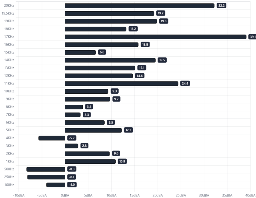
Cooler Master HAF II 500 > Noise Dampening Performance - LAeq
