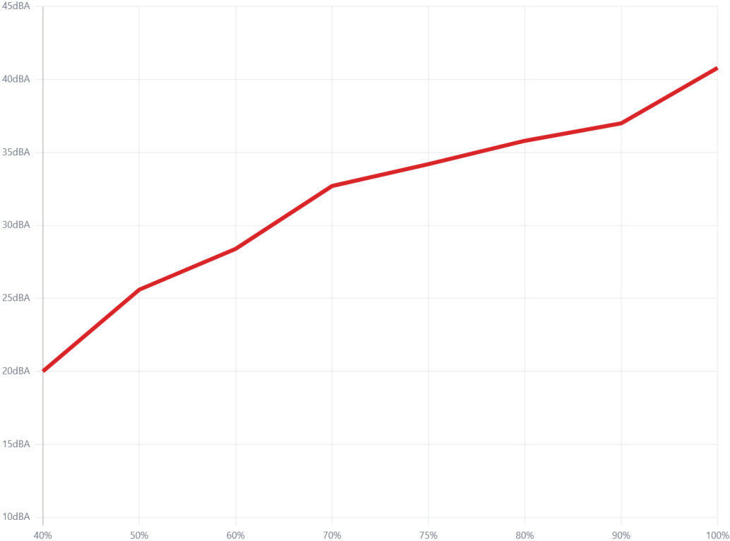
Cooler Master HAF II 500 > Stock Fans Noise Output - LAeq
