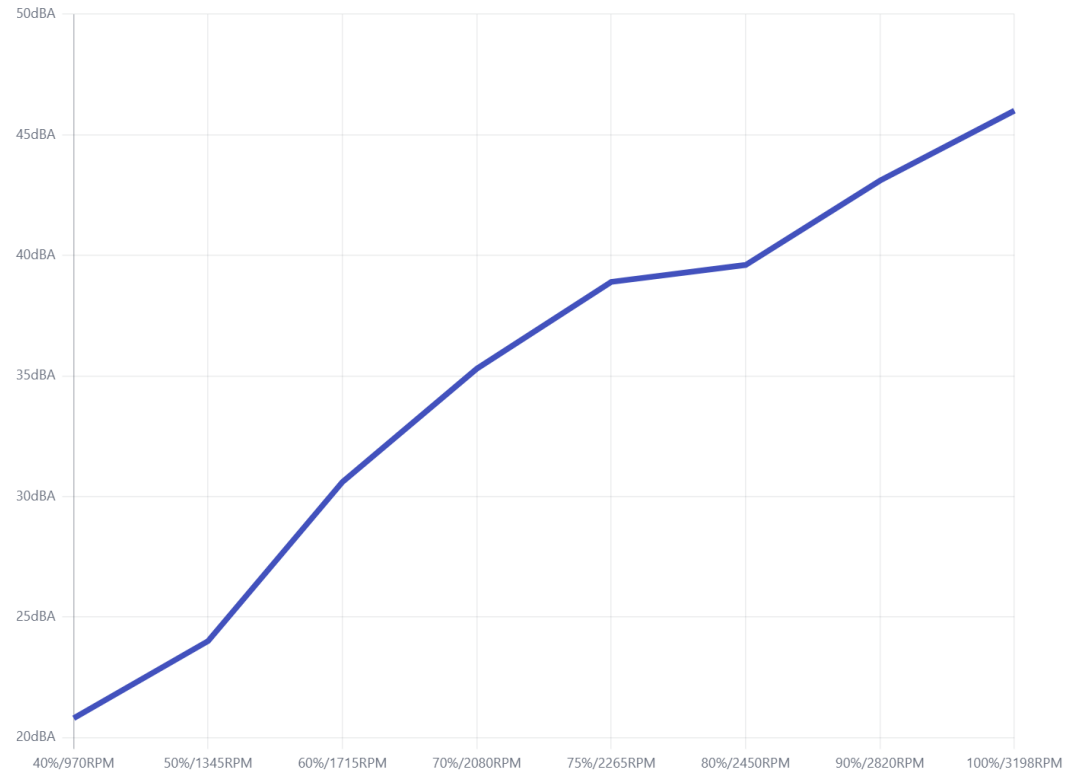
Cooler Master HAF II 500 > GPU Noise Output
