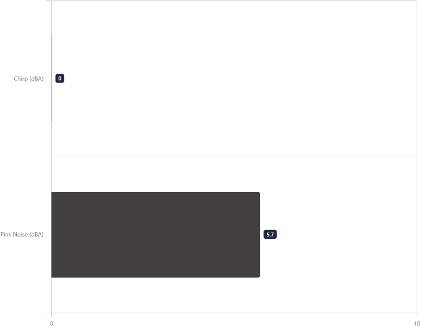
Cooler Master HAF II 500 > Noise Dampening Performance - LZeq Higher is Better
