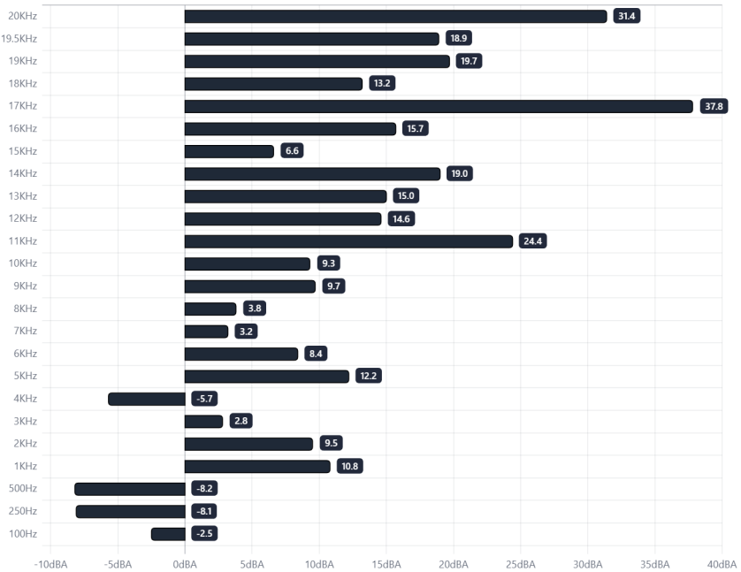
Cooler Master HAF II 500 > Noise Dampening Performance - LZeq
