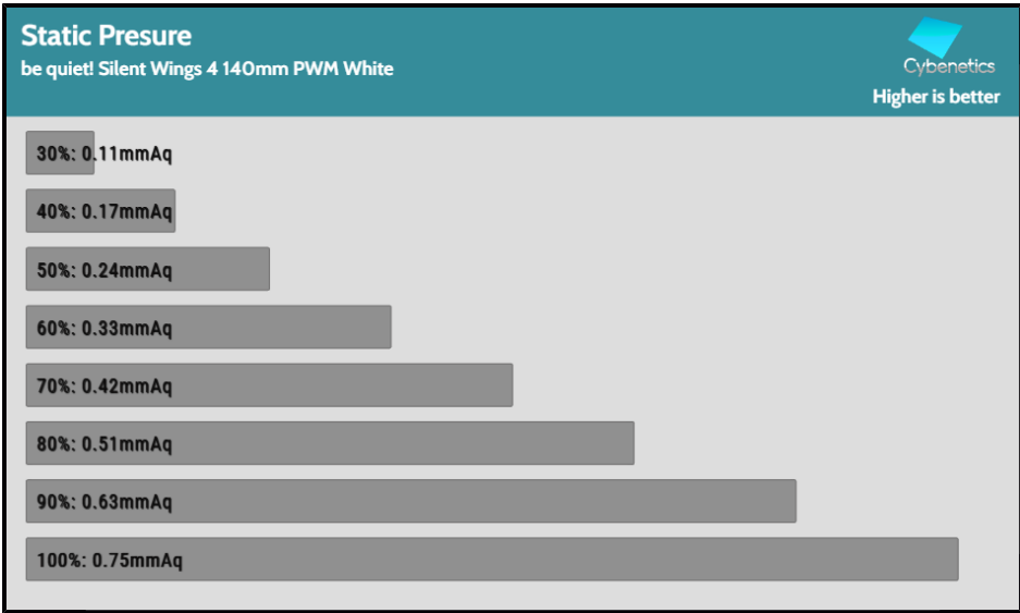
Fan Percentage Pressure
