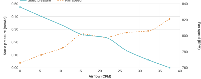
PQ Chart 3.14V
