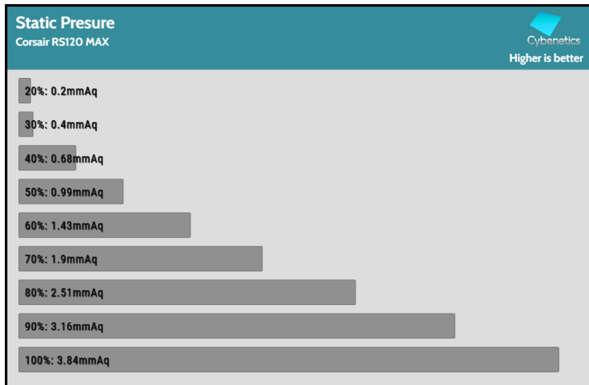
Fan Percentage Pressure
