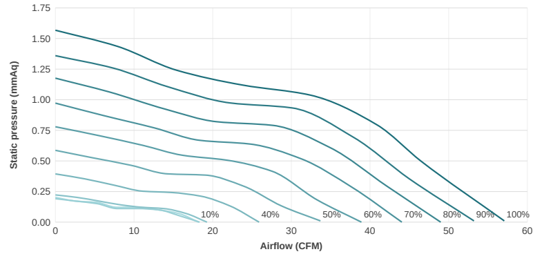
PQ Chart 10%
