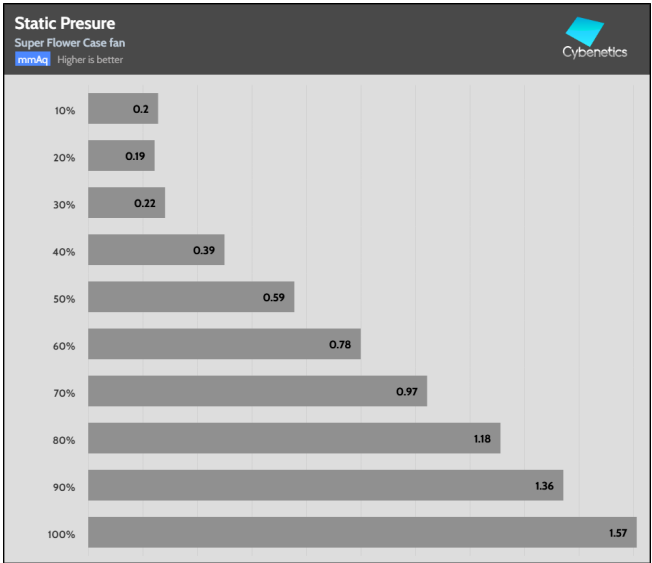
Fan Percentage Pressure
