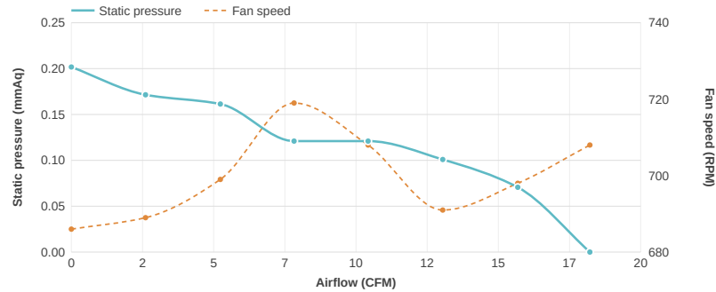
PQ Chart 10%
