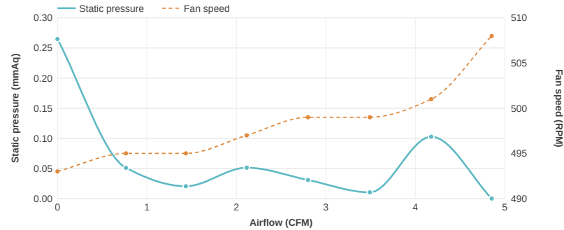
PQ Chart 20%
