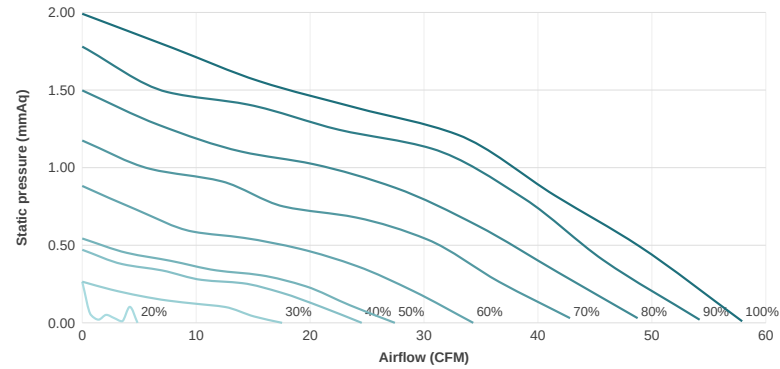
PQ Chart 20%
