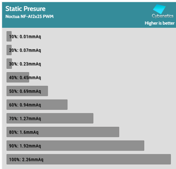
Fan Percentage Pressure
