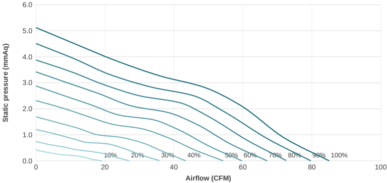
PQ Chart 10%
