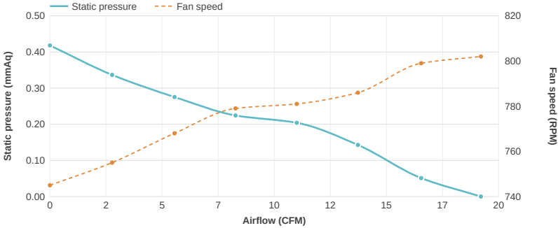
PQ Chart 10%
