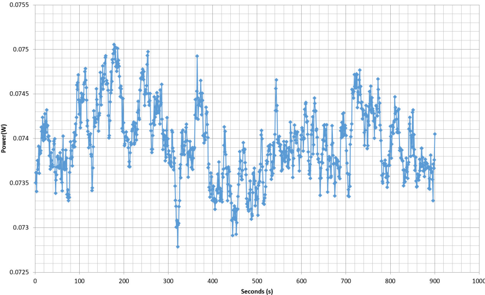
Power - R1906AA252140121 - 13/12/2019 - 11:18
