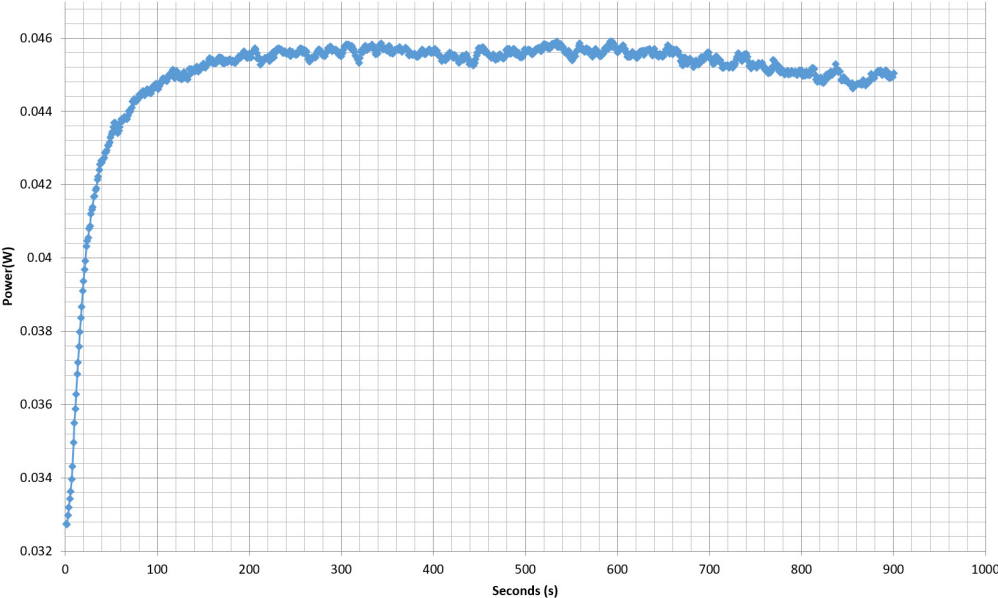
Power - R1906AA252140121 - 13/12/2019 - 11:18
