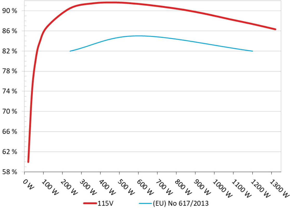
Efficiency: ASUS Rog Thor 1200W Ambient: 37°C - 47°C (98.6°F - 116.6°F)
