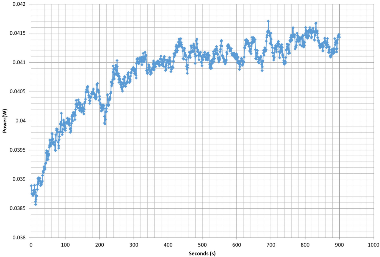
Power - PSTPG1200F1FAPU1AL000009 - 18/10/2017 - 11:47
