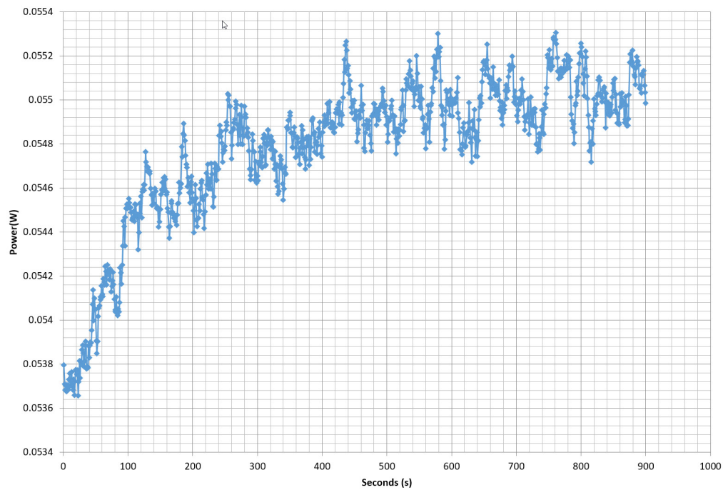
Power - R1709AA181140024 - 07/12/2017 - 13:02
