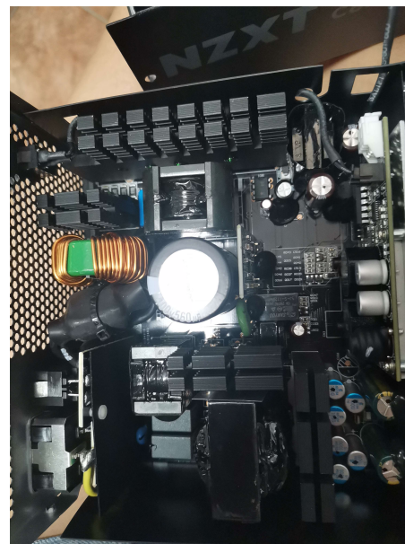
PSU Internals
