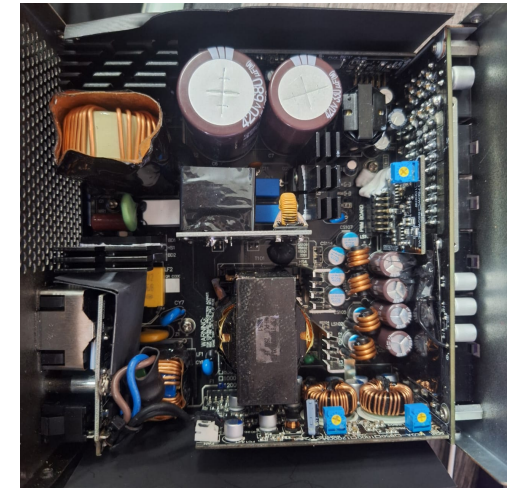
PSU Inside
