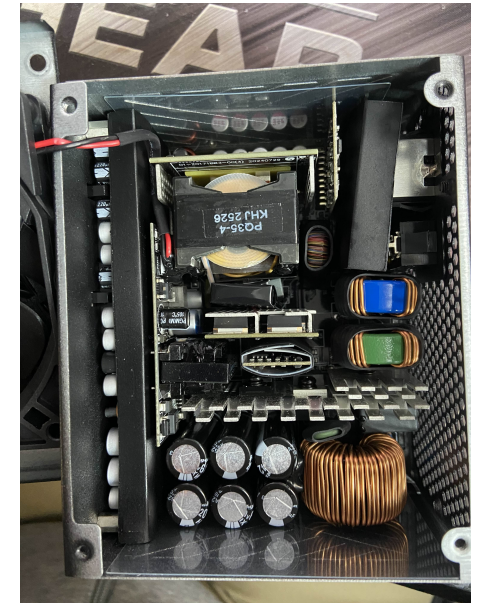
PSU Inside
