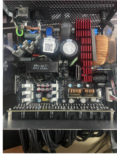
PSU Internals
