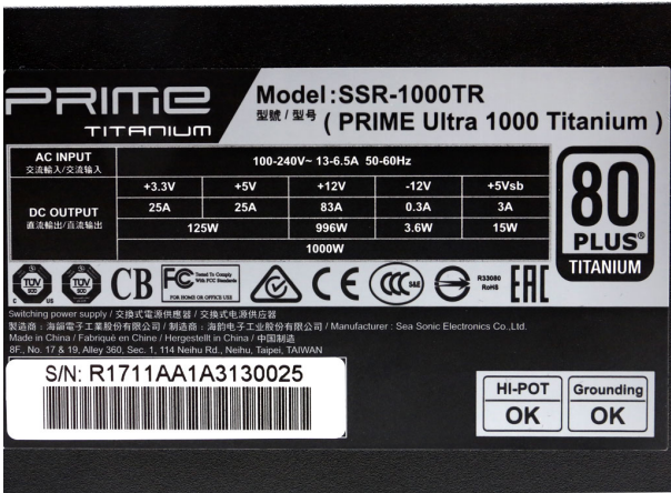
Power specifications label
