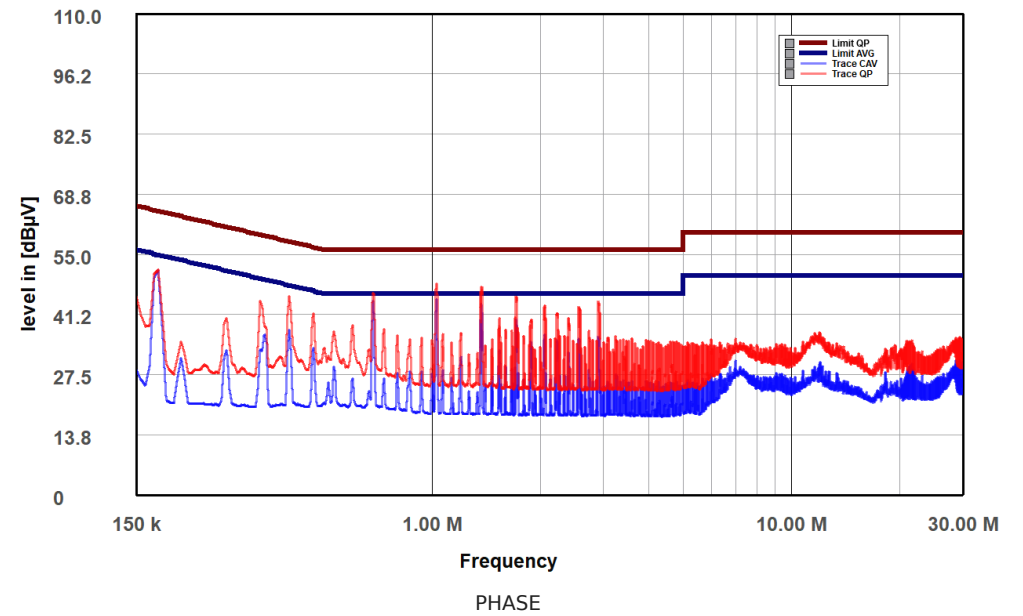
Super Flower SF-2200F14HP (SF22003003) Phase
