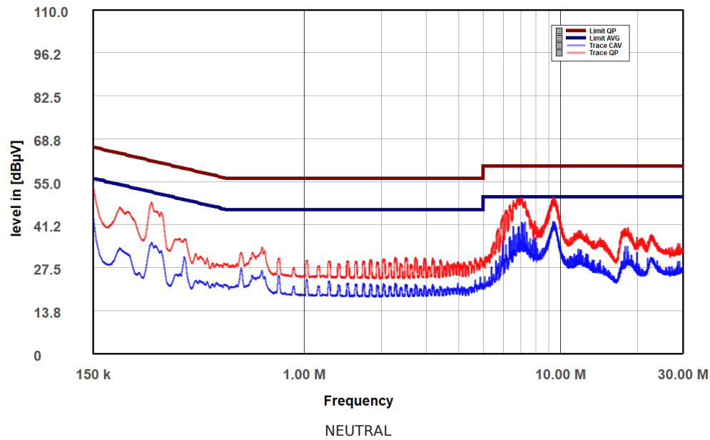
FSP Mega TI 1650 #5 (FS16503009) Neutral
