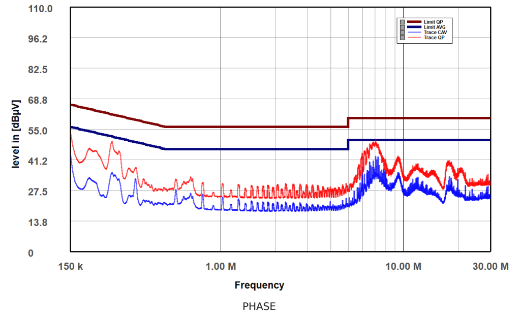
FSP Mega TI 1650 #5 (FS16503009) Phase
