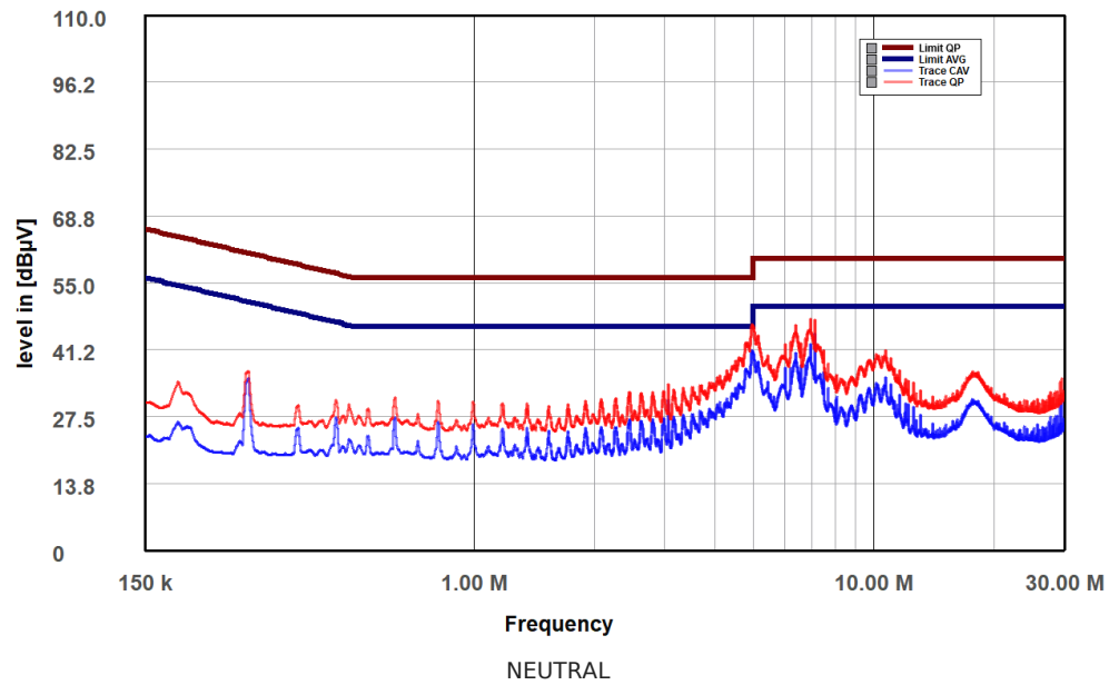
MSI MPG A1250GS PCIE5 #4 (MS12503023) Neutral
