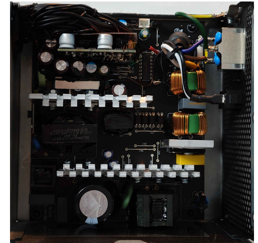
PSU Internals
