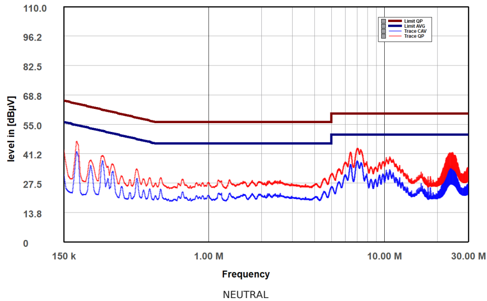
XPG Pylon II 550 (AD55003027) Neutral
