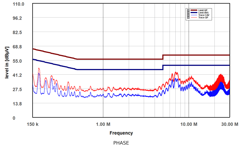
XPG Pylon II 550 (AD55003027) Phase
