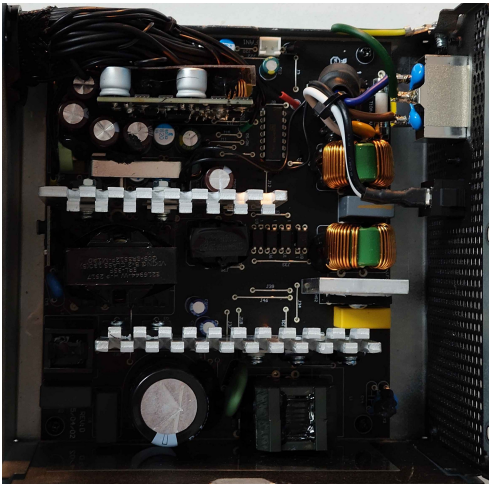
PSU Internals
