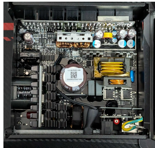
PSU Internals
