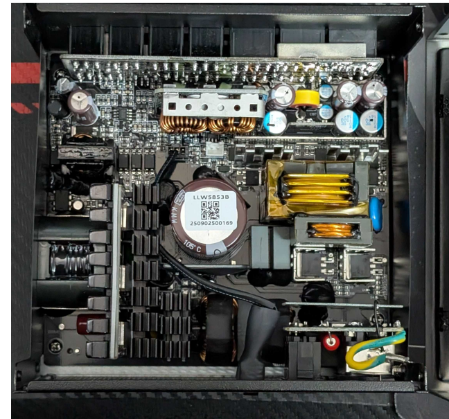
PSU Internals
