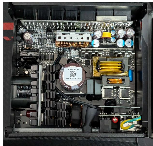
PSU Internals
