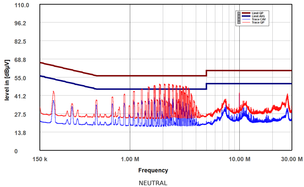
Gigabyte AE1000PM PG5 (GB10003053) Neutral
