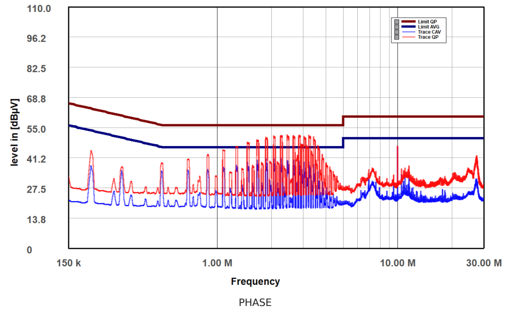
Gigabyte AE1000PM PG5 (GB10003053) Phase
