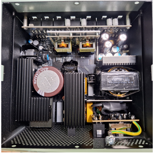
PSU INTERNAL
