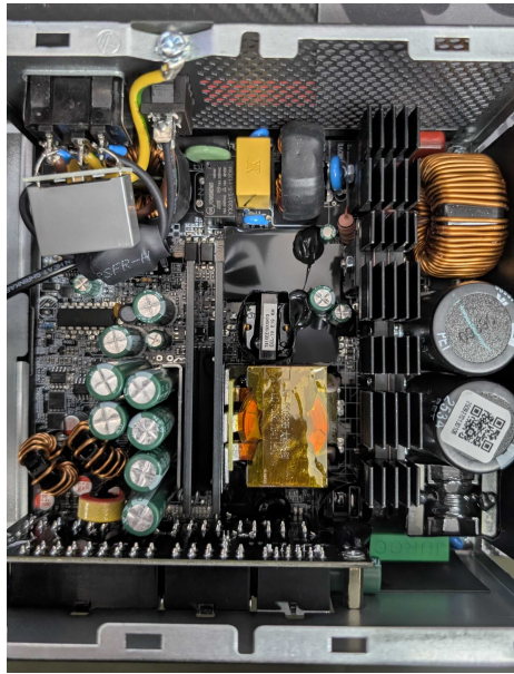
PSU Internals
