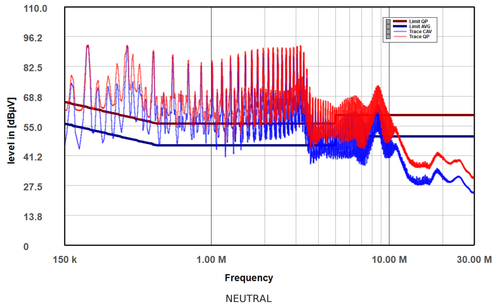
Wentai AiBarza Aldan-D1515 (WT13003083) (WT15103082) Neutral
