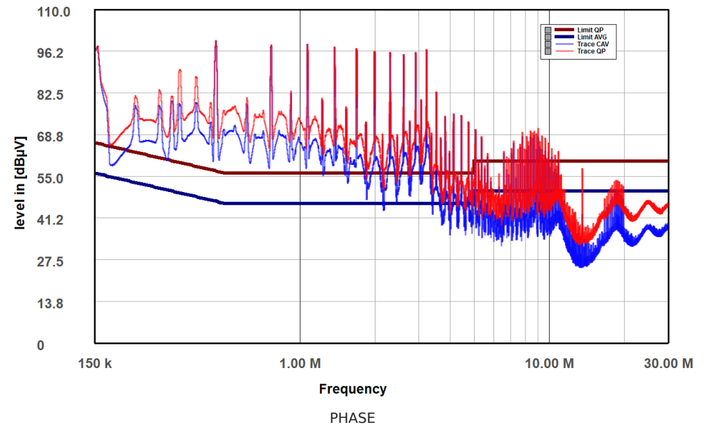
Wentai AiBarza Aldan-D1515 (WT13003083) (WT15103082) Phase
