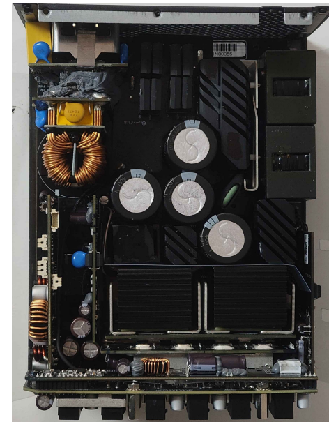
PSU Internals
