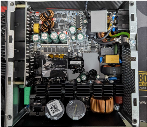
PSU Internals
