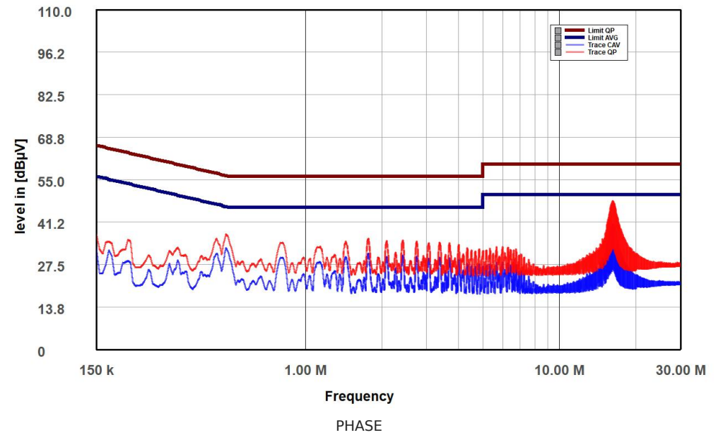
ASRock Steel Legend SL-1200P (AR12003095) Phase
