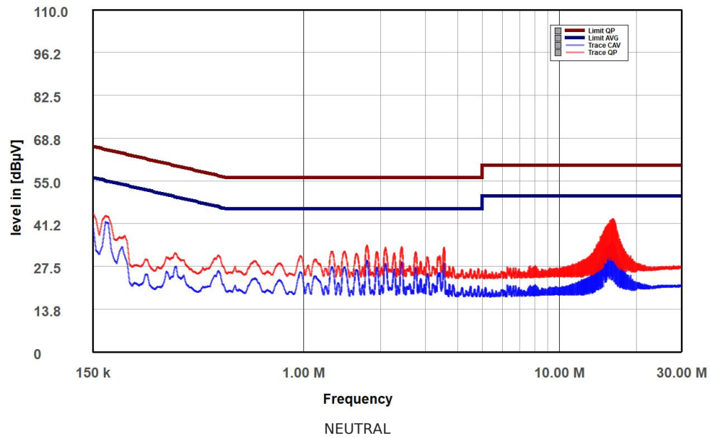
ASRock Steel Legend SL-1200P (AR12003095) Neutral
