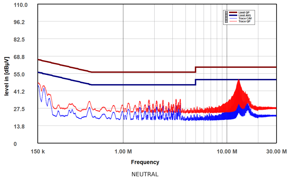
ASRock Steel Legend SL-1000P (AR10003098) Neutral
