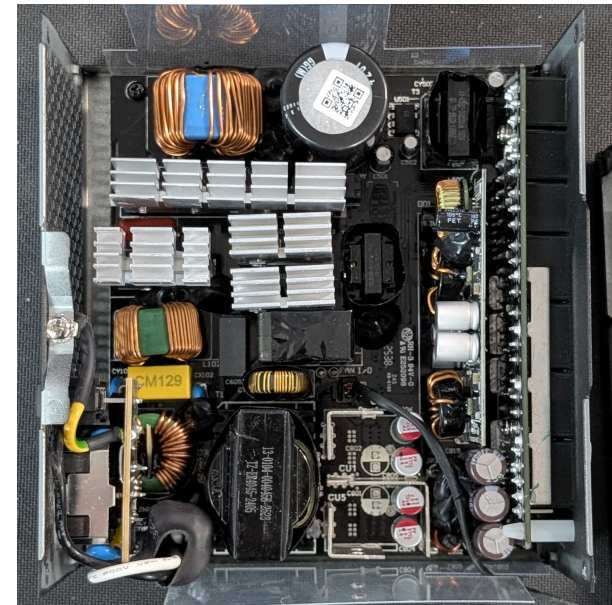
PSU Internals
