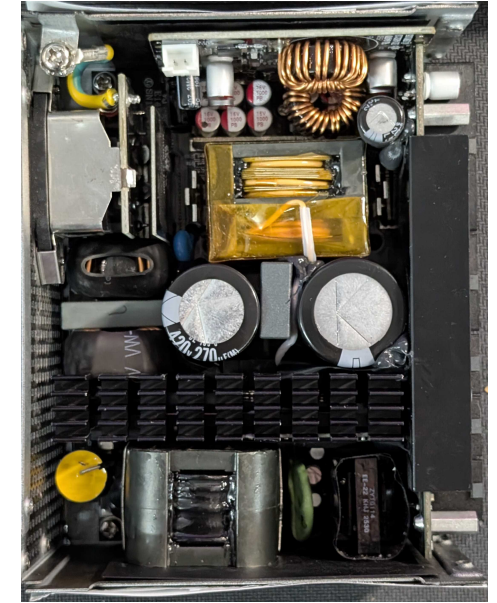
PSU Internals
