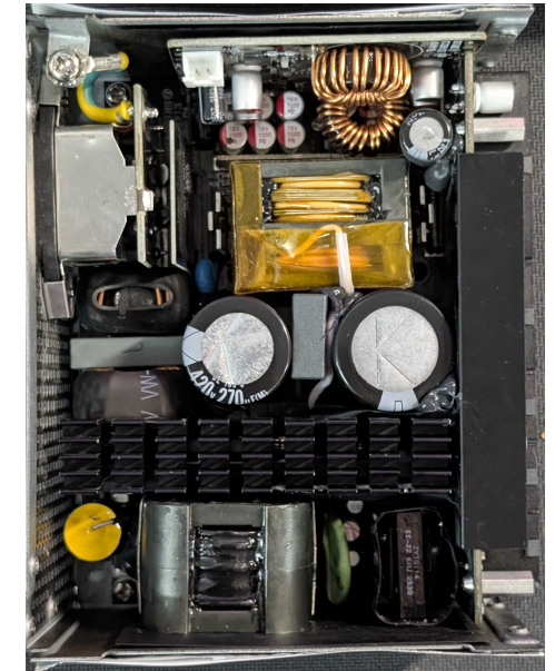
PSU Internals
