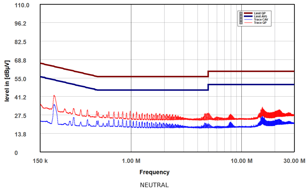
MSI MAG A1200PLS PCIE5 (MS12003120) Neutral
