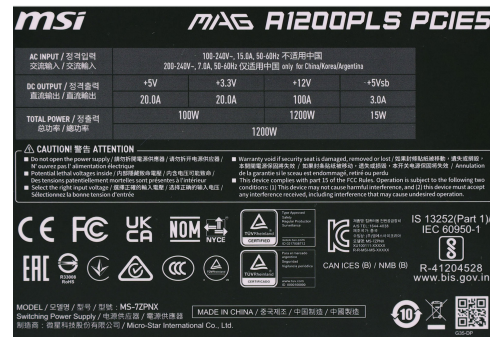
Power specifications label
