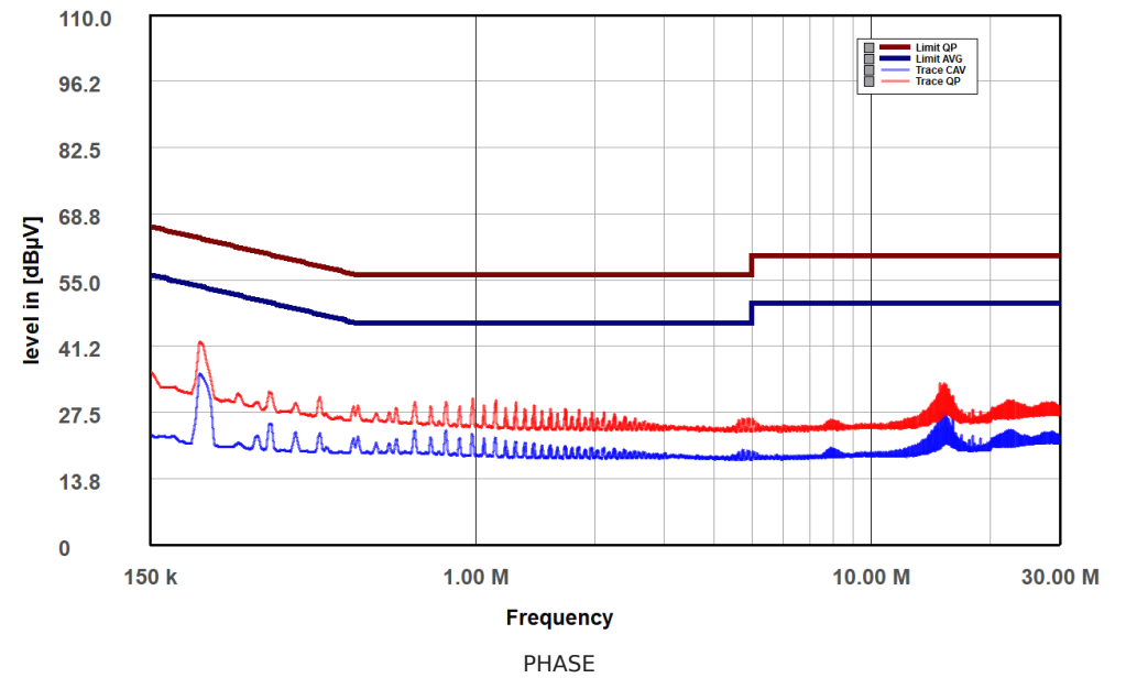
MSI MAG A1200PLS PCIE5 (MS12003120) Phase
