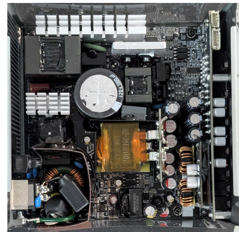
PSU Internals
