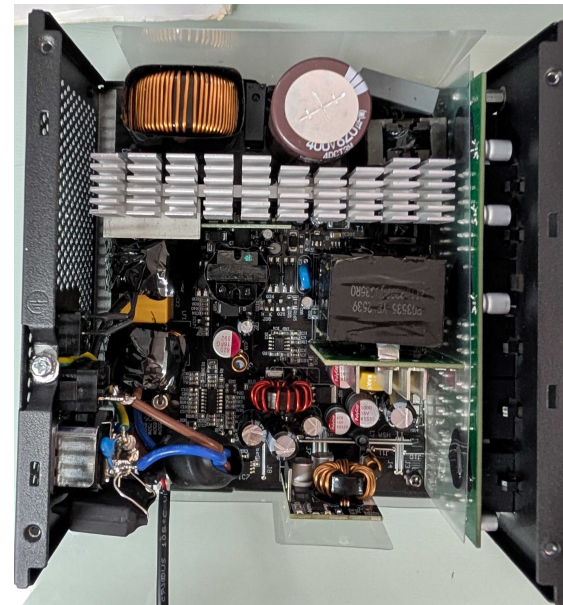
PSU Internals
