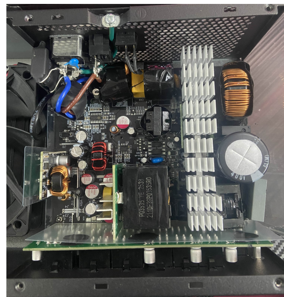
PSU Internals
