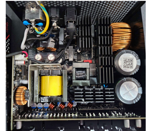
PSU Internals
