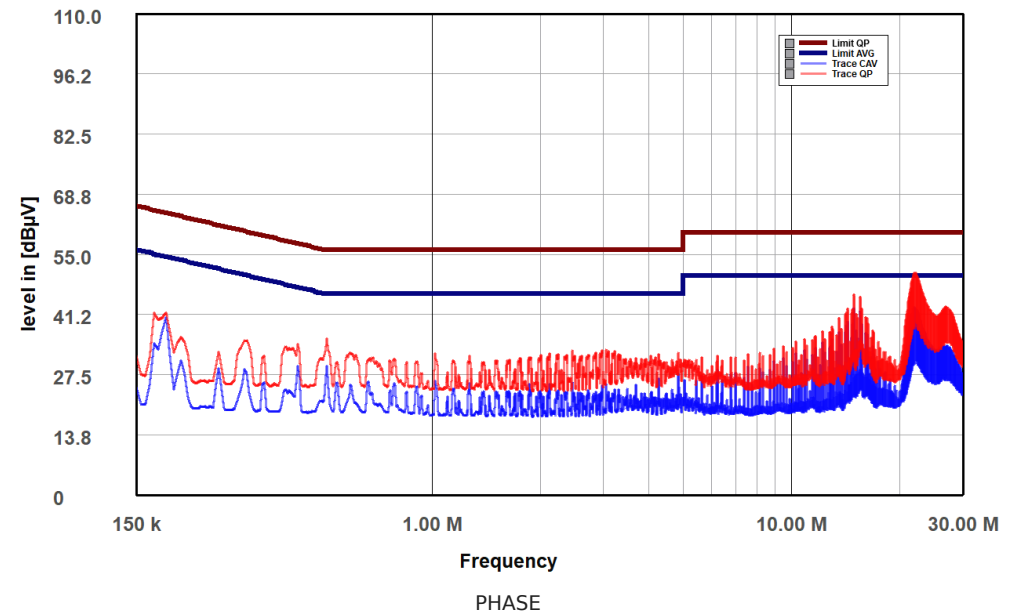
Sharkoon Rebel P20 Gen 2 750W (SK75003156) Phase
