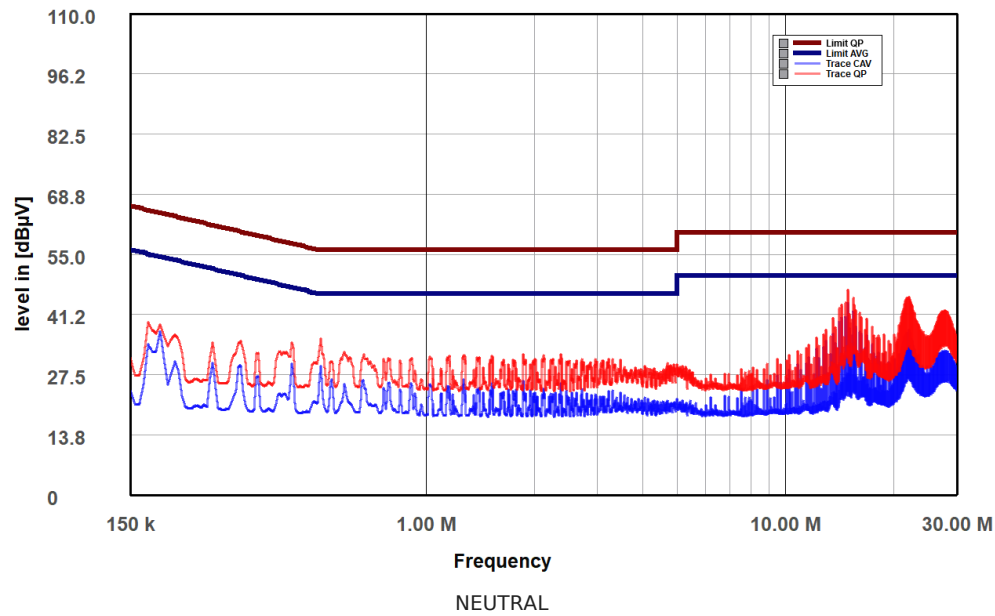
Sharkoon Rebel P20 Gen 2 750W (SK75003156) Neutral
