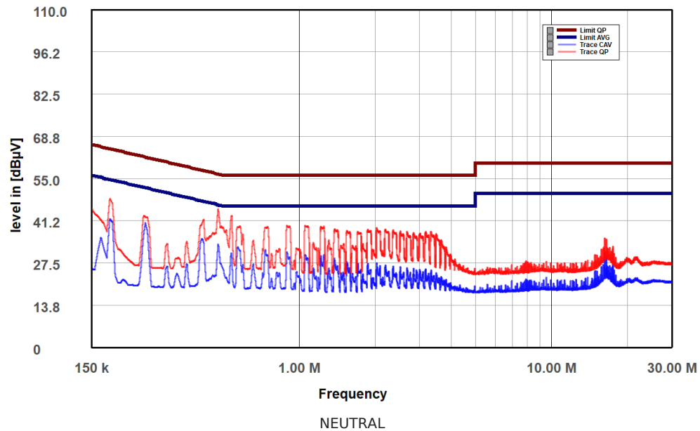
Thermaltake Toughpower TF3 1650W (TT16503181) Neutral
