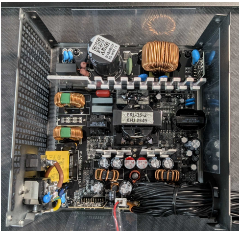
PSU Internals
