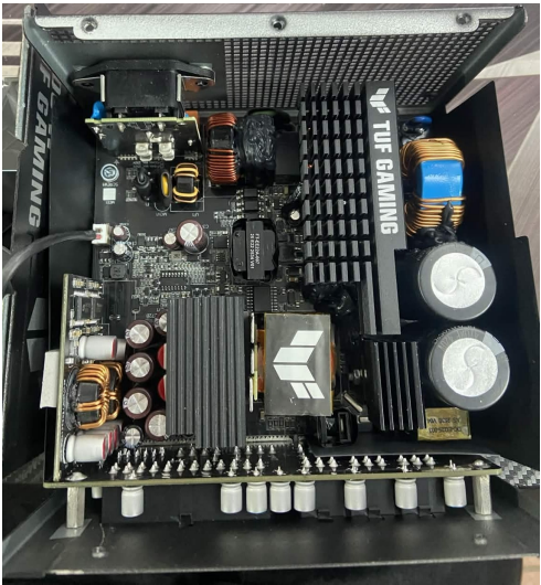
PSU Internals
