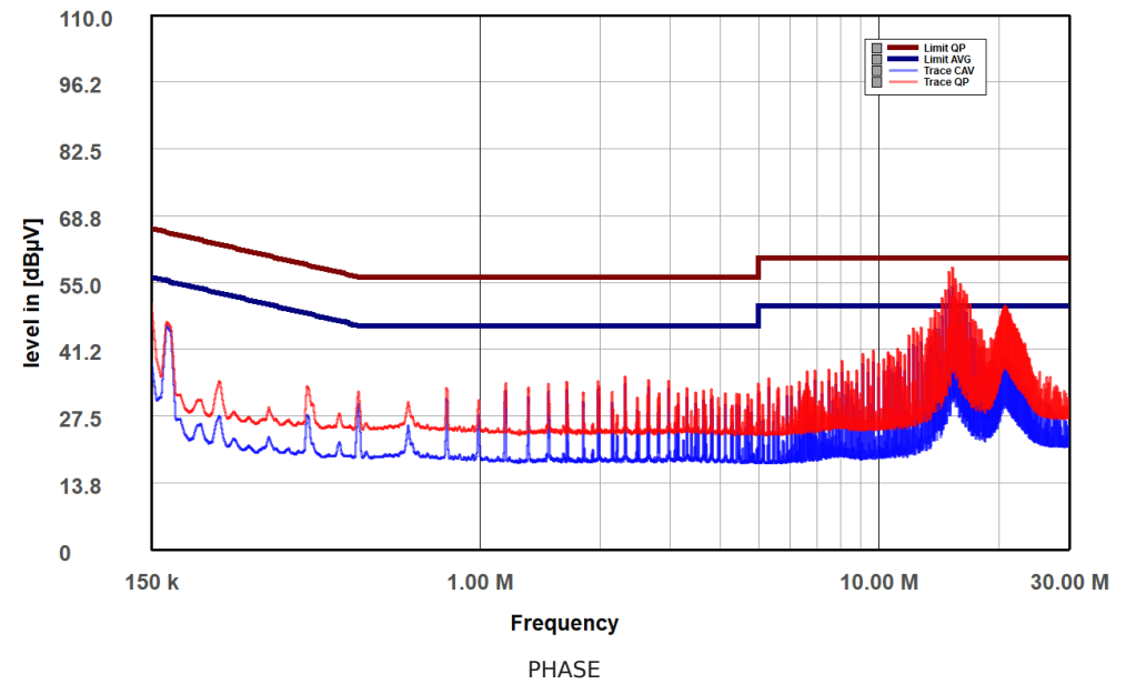
Asus Tuf Gaming 1200W (AS12001231) Phase
