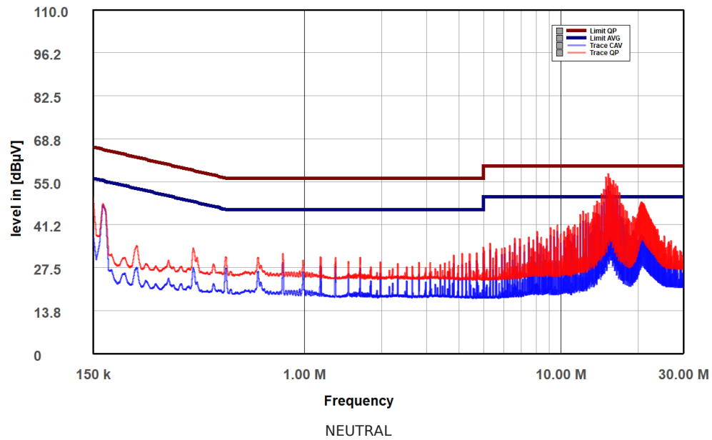
Asus Tuf Gaming 1200W (AS12001231) Neutral
