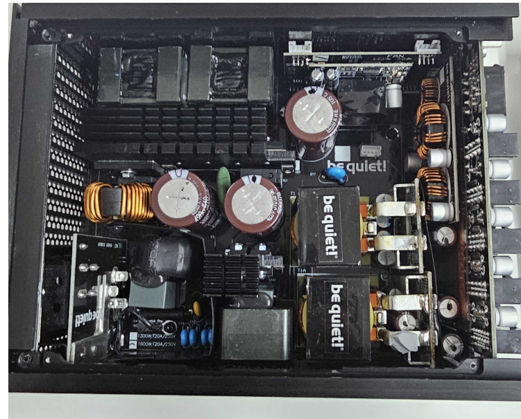
PSU Internals
