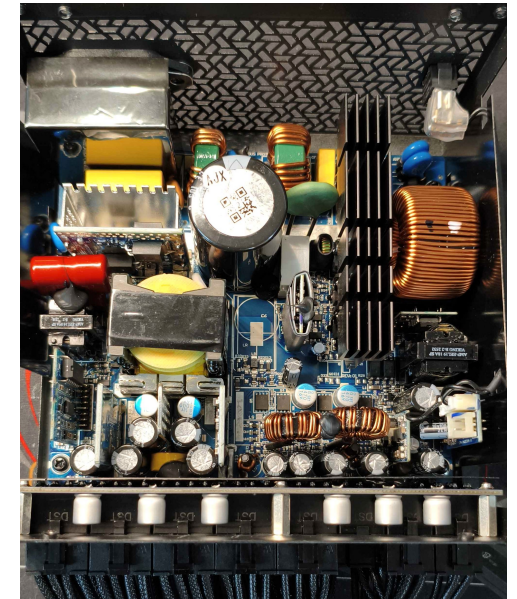
PSU Internals
