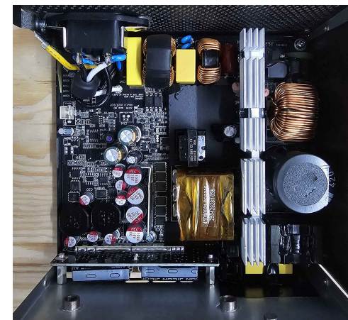
PSU Internals
