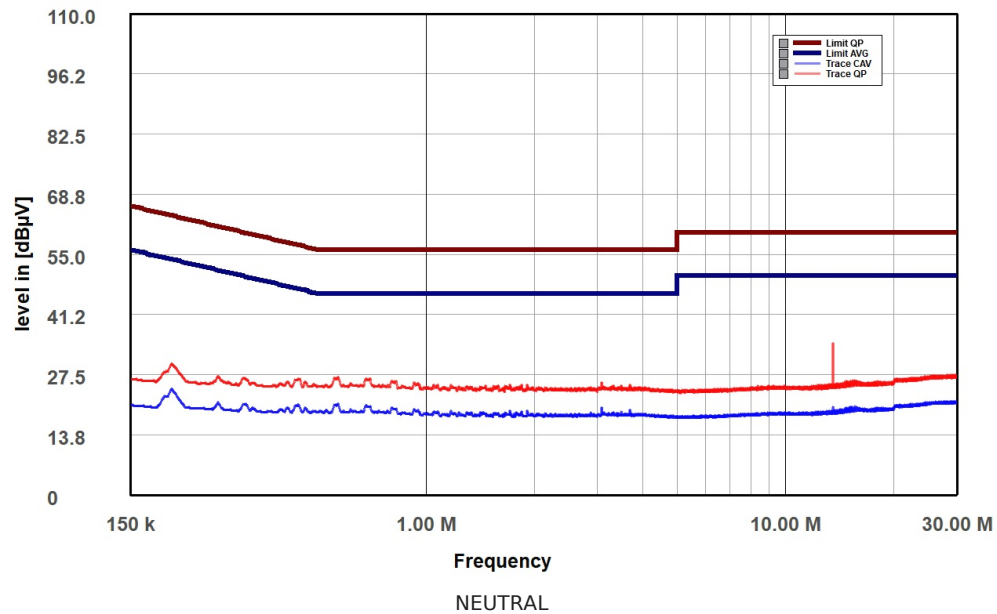
Thermaltake Dockpower FI 750W (TT75003416) Neutral
