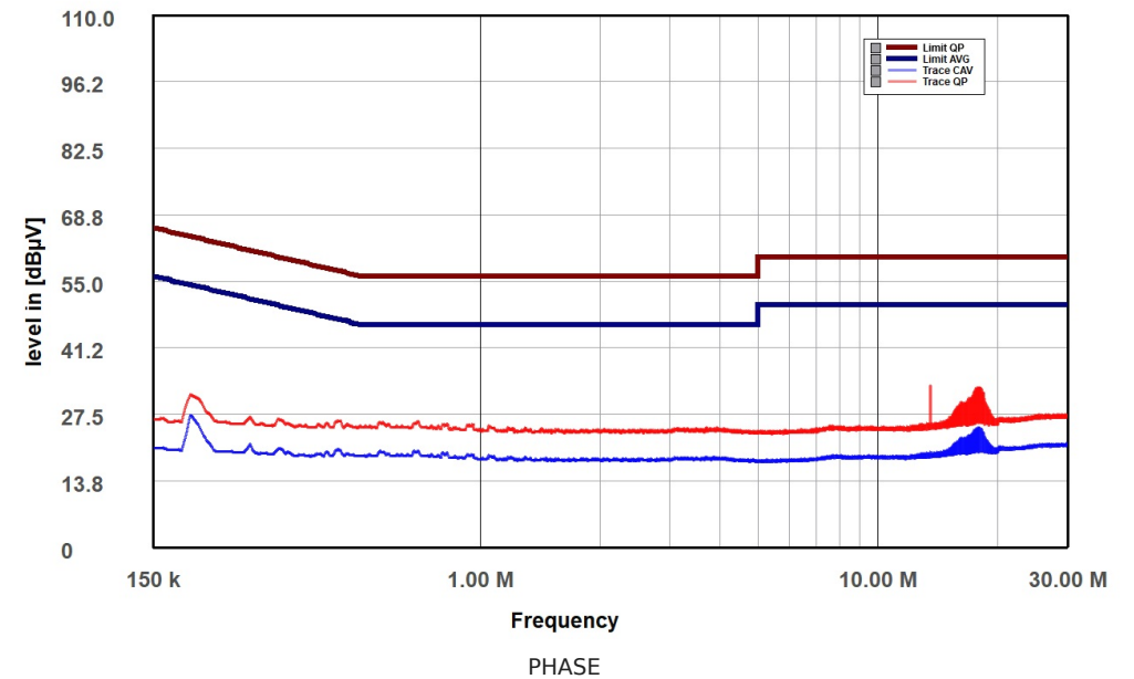
Thermaltake Dockpower FI 750W (TT75003416) Phase
