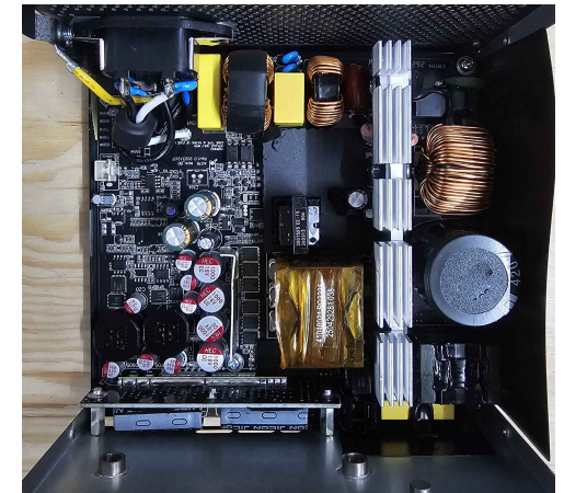
PSU Internals
